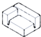
Left Module 120 Cod. OLEMC120 W 128 D 100 H 66 cm H seat 44 cm
